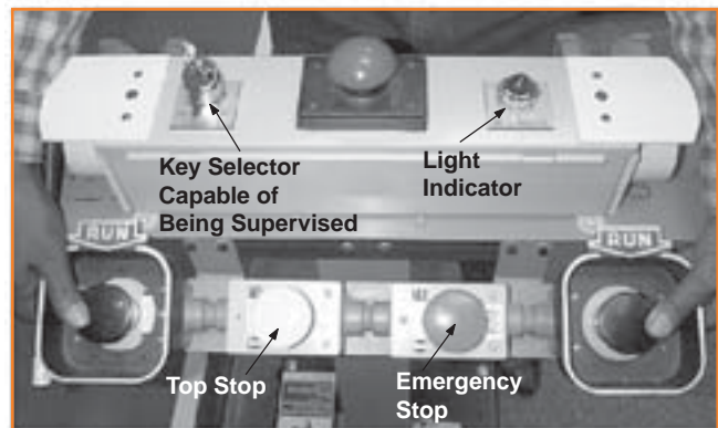
Figure 17. Two-Hand Control
