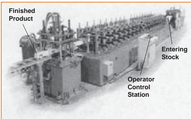
Figure 33. Roll-Forming Machine
