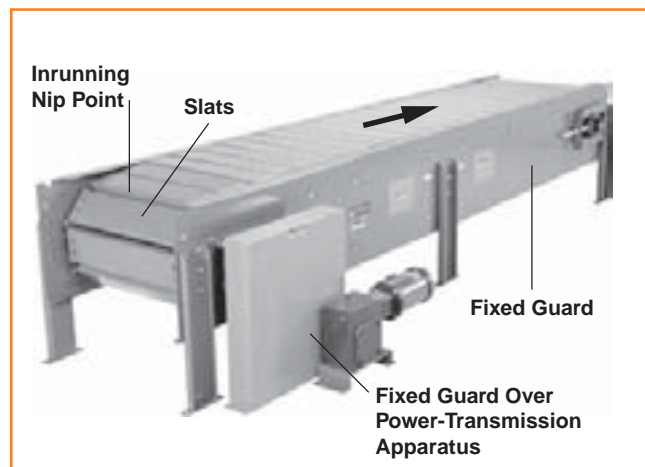
Figure 30. Slat Conveyor
